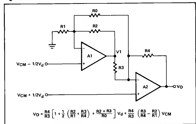
FIGURE 1: Two-Op-Amp Instrumentation Amplifier Configuration
